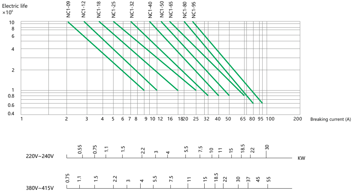
Rated outputs of three-phase motors (50Hz AC-3)
