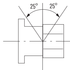
Figure 25 - Mounting Position – 100S-C DC Contactors with Conventional Coils
