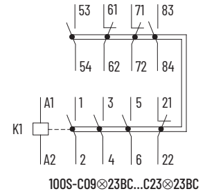
Figure 10 - Safety Reversing Contactors with 3 Main Contacts and Bifurcated Front-mount Auxiliary Contacts
