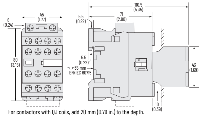
Figure 39 - 100-E09...100-E16 Contactors with Low-consumption Coils and Front-mounted Auxiliary Contact
